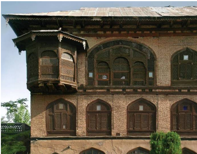
Fig. 1 Detail of the Jalali Haveli, Srinagar, Kashmir, India, ca. 1860. This is a timber-laced bearing wall masonry structure known as taq construction in India and bhatar construction in Pakistan. The timber lacing at the floor levels is visible on the exterior as part of the architectural expression.
