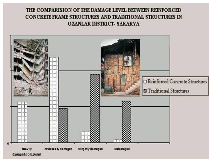
Fig. 6 A graph from the report by Turkish researchers D. Gulhan and I.Ö. Gunay showing a statistical comparison between the performance of buildings of traditional forms of masonry construction and reinforced concrete frame construction in one district in the heart of the damage district after the first of the 1999 earthquakes in Turkey. [2] (The photos of examples were added.)
