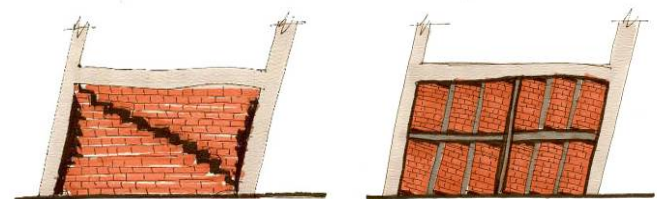
Fig. 8 These diagrams show the conceptual difference between the earthquake performance of a standard masonry infill wall (left) and an Armature Crosswall (right) in reinforced concrete frame construction. The sub-frame (which in modern construction can be of any material including concrete or steel, not only timber), holds the brick masonry panels in place, allowing the deformation of the system without the likelihood of the development of diagonal tension “X” cracks that can lead to the rapid collapse of the wall. An important component of the Armature Crosswall system is the use of mortar that is soft and weaker than the masonry units, such as lime or clay mortar rather than cement mortar. The initial stiffness of the standard infill wall, which is usually laid up with cement mortar, also can cause the surrounding frame to be broken leading to its collapse, while the Armature Crosswall is much less stiff at the onset of shaking, allowing “frame action” to take place.
